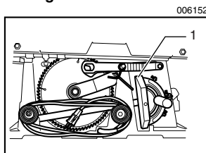
1. Miter gauge
